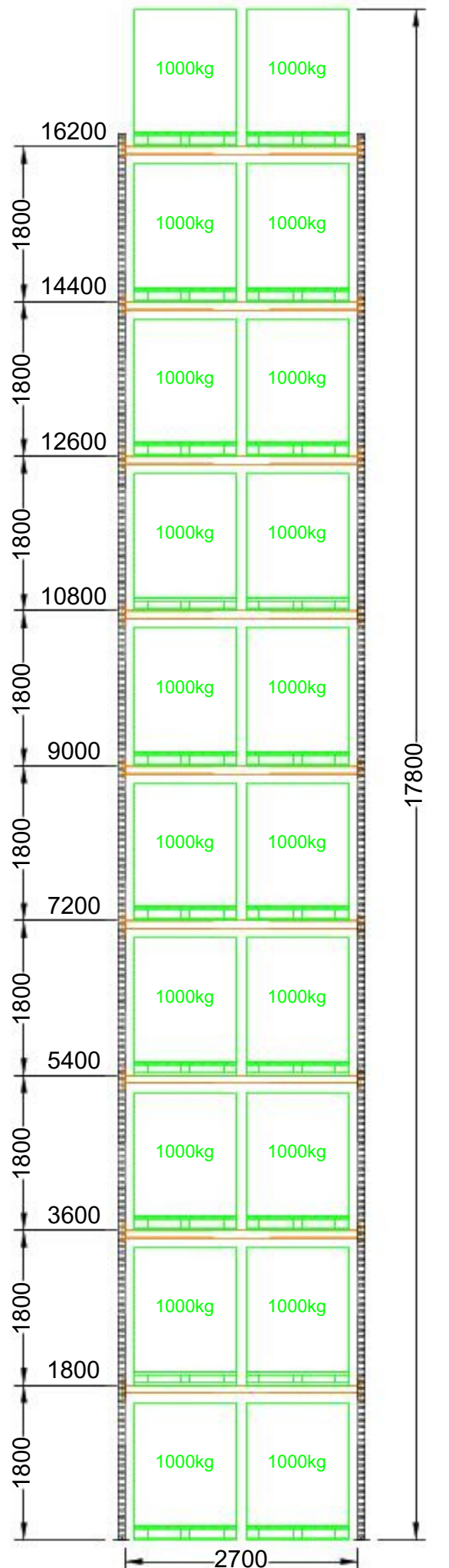
TYPICAL BAY ELEVATION
