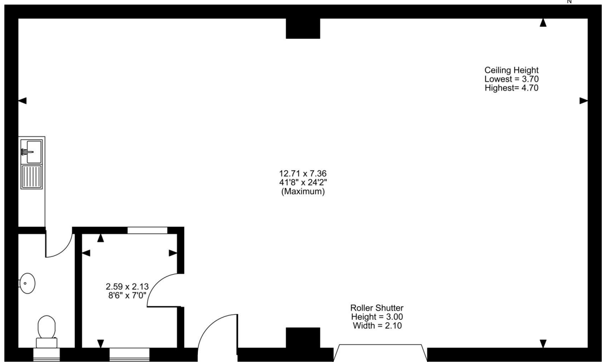
Ground Floor
